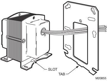
Fig. 7. Tab on mounting plate fits in slot on transformer mounting foot.
