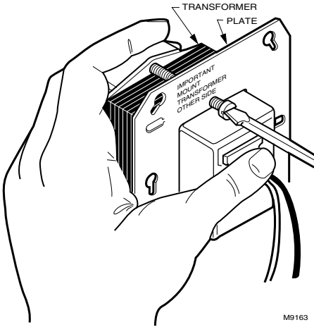
Fig. 8. Secure plate to transformer with mounting screw.
