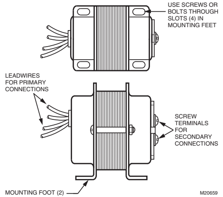
Fig. 10. Foot mounting of AT87 Transformer.
