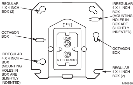
Fig. 9. Location of mounting holes.
