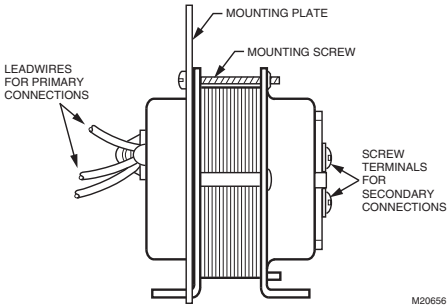
Fig. 4. Plate may be mounted to transformer in one of two positions (AT72D shown).
