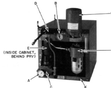
A-4400 Series Refrigerated Air Dryer with Cover
